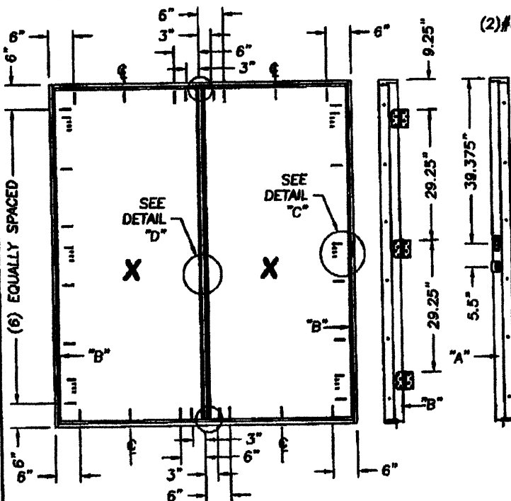
ALUMINUM ASTRAGAL
