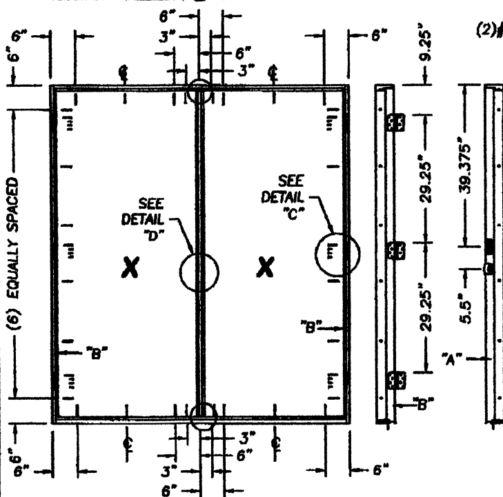
ALUMINUM ASTRAGAL
